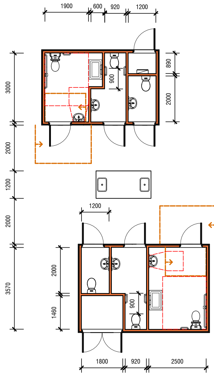
OPTION 02 - FLOOR PLAN LAYOUTS
